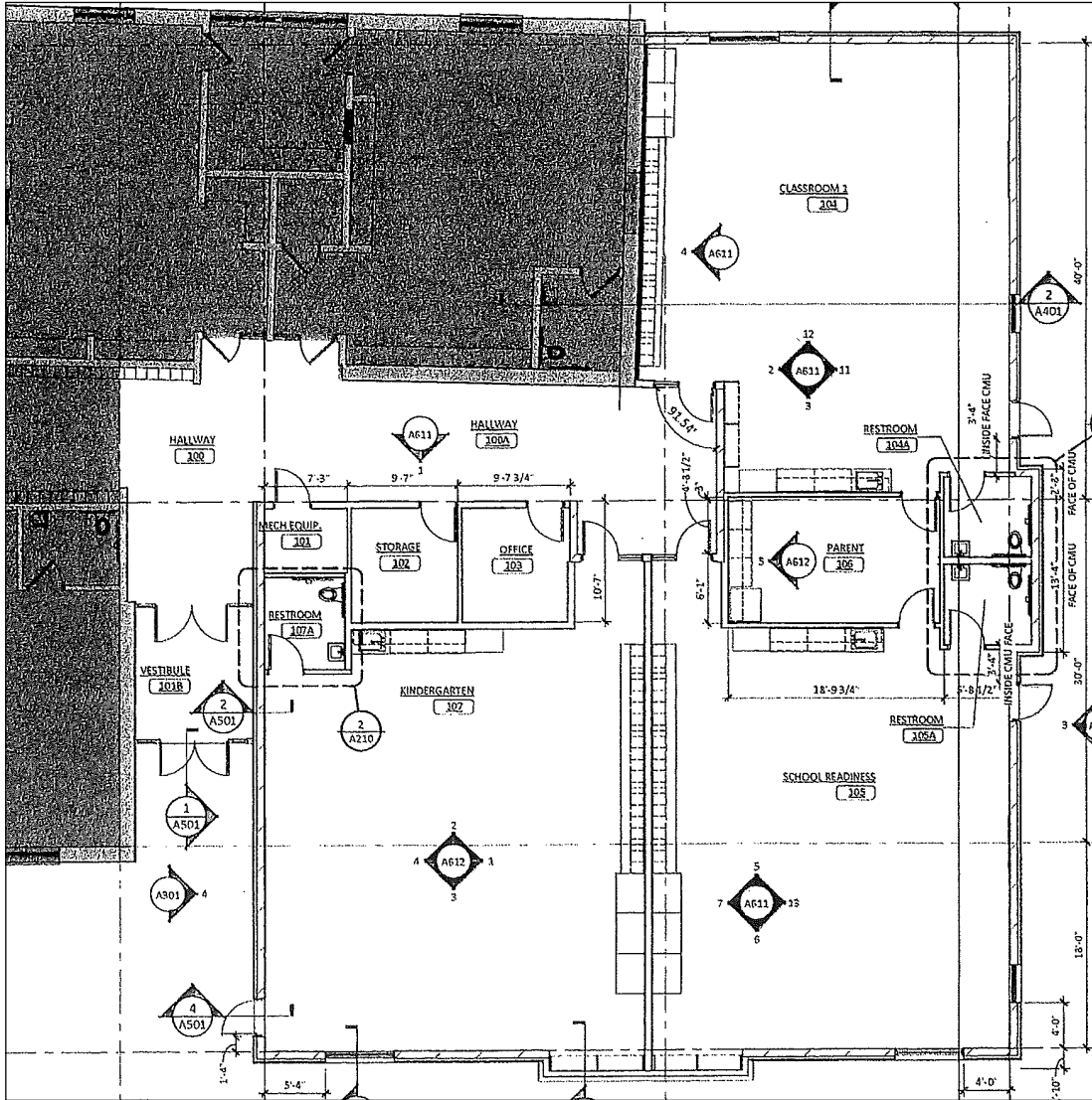
Final drawings for the new addition to the east end of the Clearbrook-Gonvick School were approved. The dark areas show the existing classrooms to the west. The hallway and vestibule where the three rooms would be connected.
